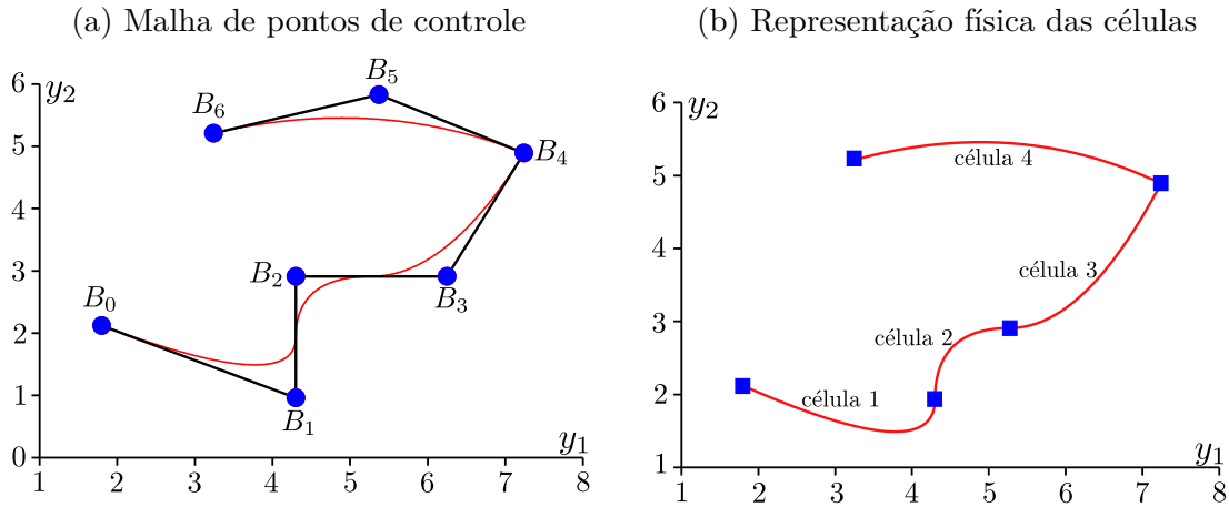
Figura 17 – Curva B-Spline
